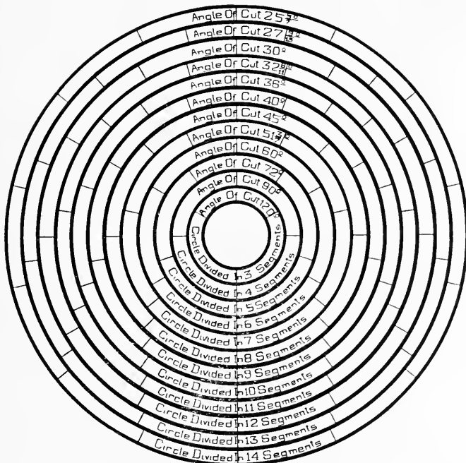
FIG. 210. TABLE FOR SEGMENTAL WORK WITH TRIMMER.
